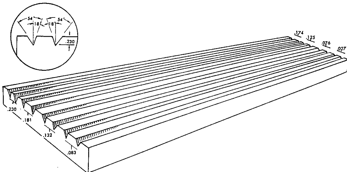
5-Strip Planing and 6-Strip Planing Form
