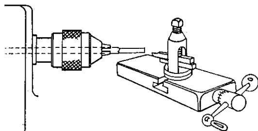
Workbench—Turning Ferrule Diameter
